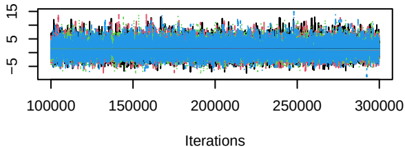
Trace of d.chemo.Gefitinib
