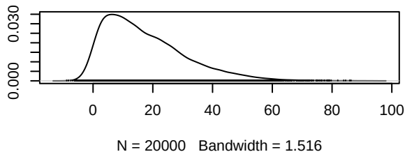
Density of d.Erlotinib.Erlotinib_MMPi
