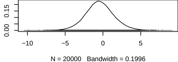
Density of d.Osimertinib.Lazertinib_Amivantamab
