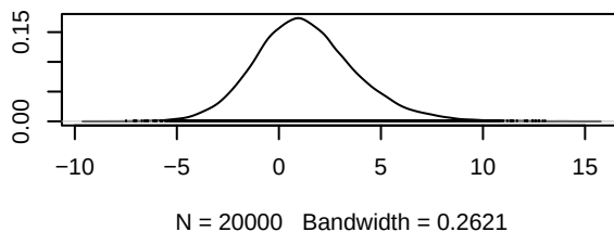
Density of d.chemo.Gefitinib
