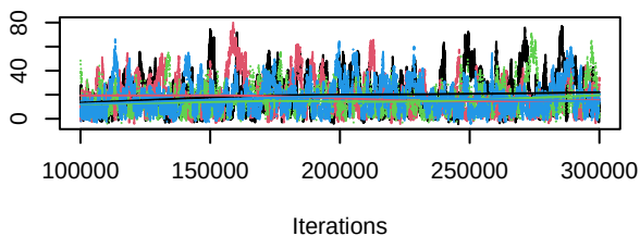
Trace of d.Gefitinib.Icotinib
