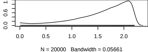
Density of sd.d
