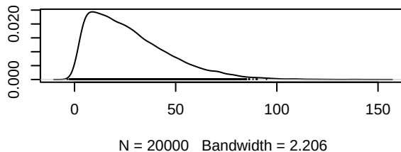
Density of d.Erlotinib.antiangio
